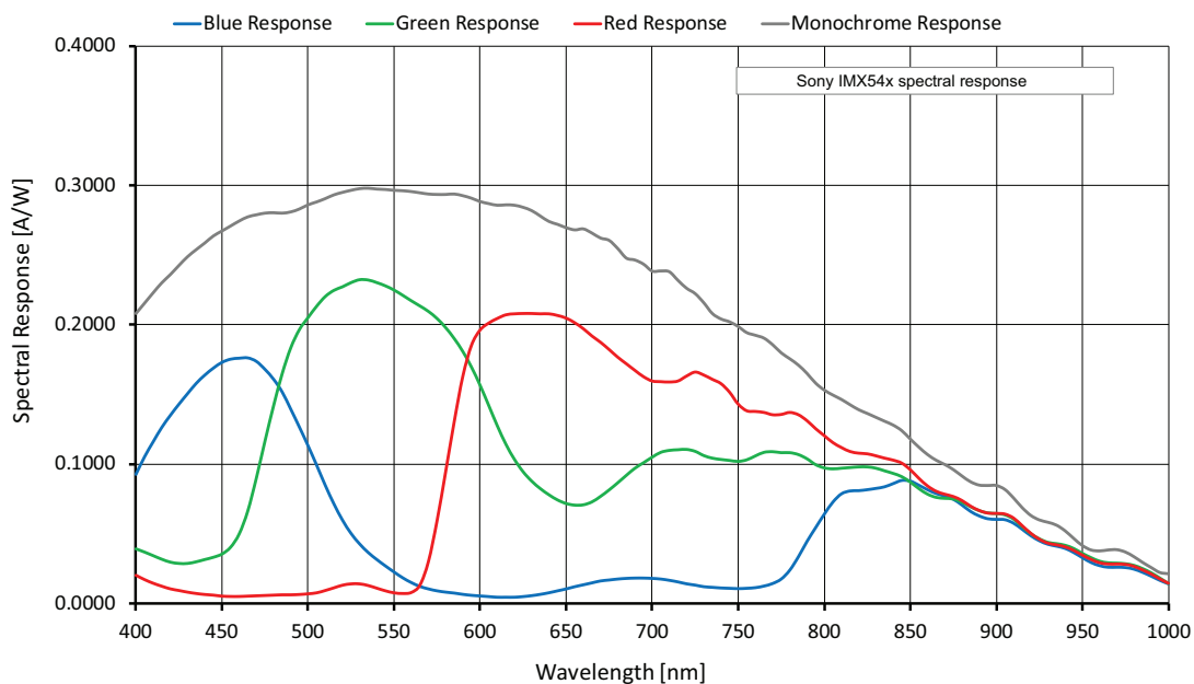
Figure 34: Alvim G1-2040m/c (Sony IMX541) spectral response
