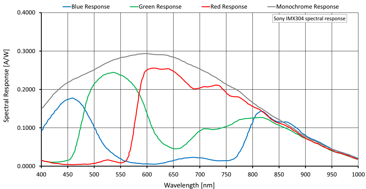
Figure 26: Alvim G1-1236m/c (Sony IMX304) spectral response
