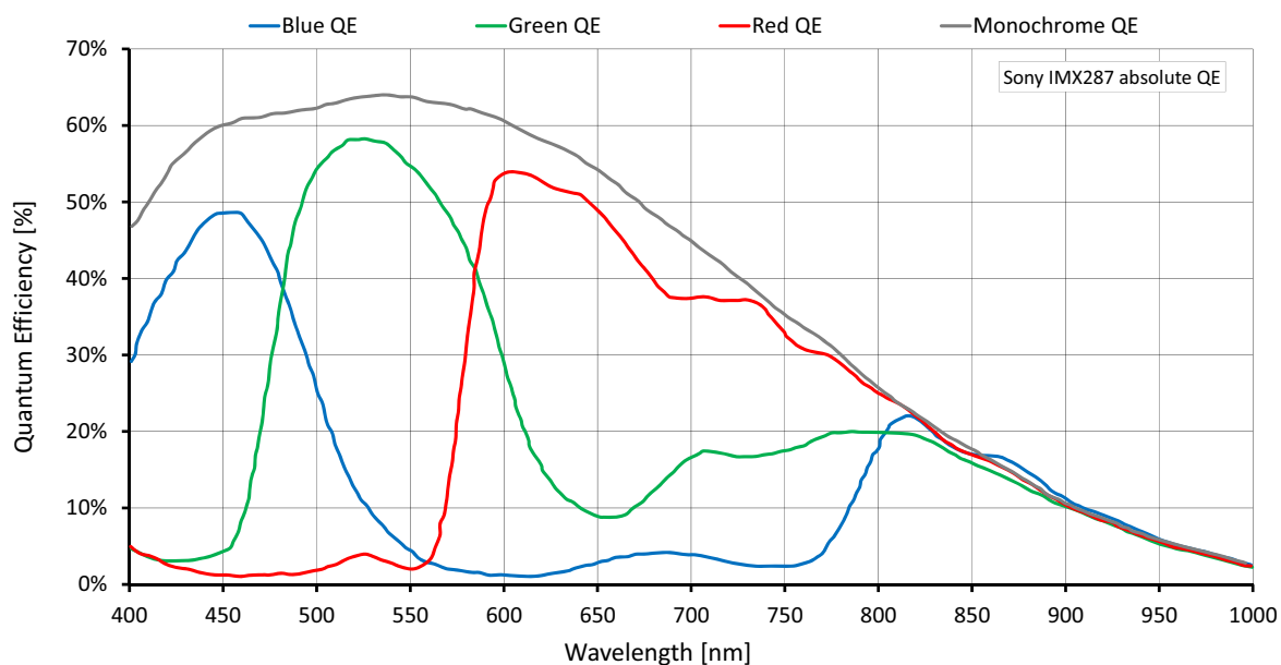
Figure 6: Alvium G1-040m/c (Sony IMX287) absolute QE
