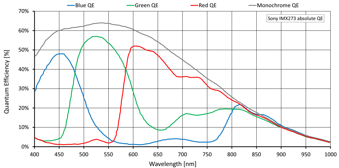
Figure 9: Alvim G1-158m/c (Sony IMX273) absolute QE
