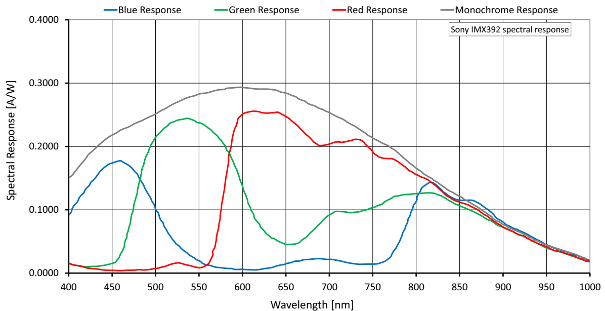
Figure 14: Alvim G1-240m/c (Sony IMX392) spectral response
