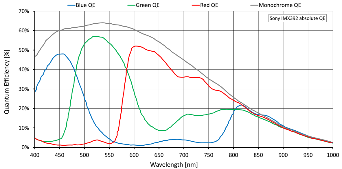
Figure 13: Alvim G1-240m/c (Sony IMX392) absolute QE
