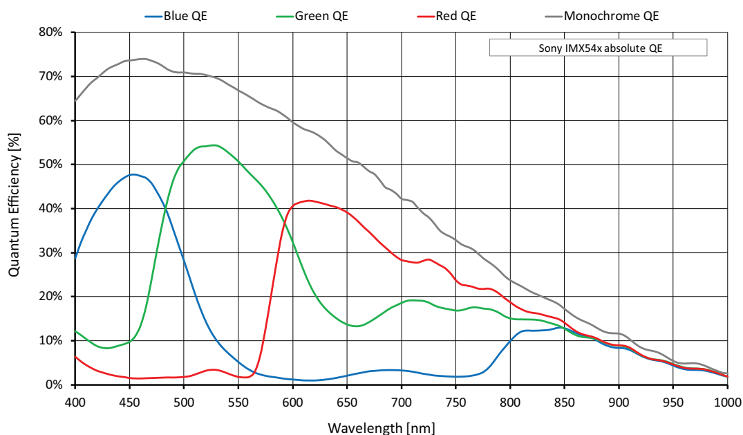
Figure 37: Alvim G1-2460m/c (Sony IMX540) absolute QE
