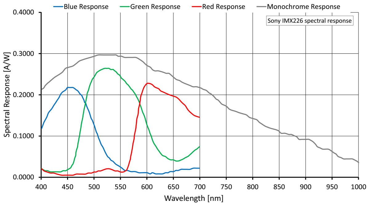
Figure 28: Alvim G1-1240m/c (Sony IMX226) spectral response
