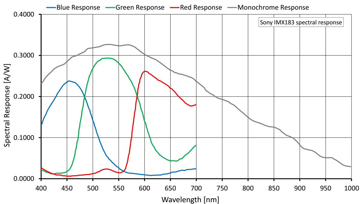
Figure 36: Alvim G1-2050m/c (Sony IMX183) spectral response
