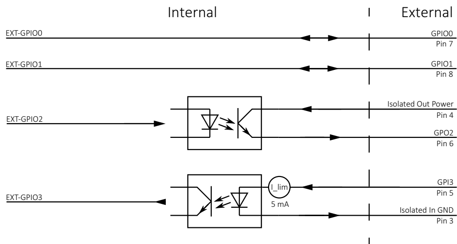
Figure 70: TFM I/O connector pin assignment
