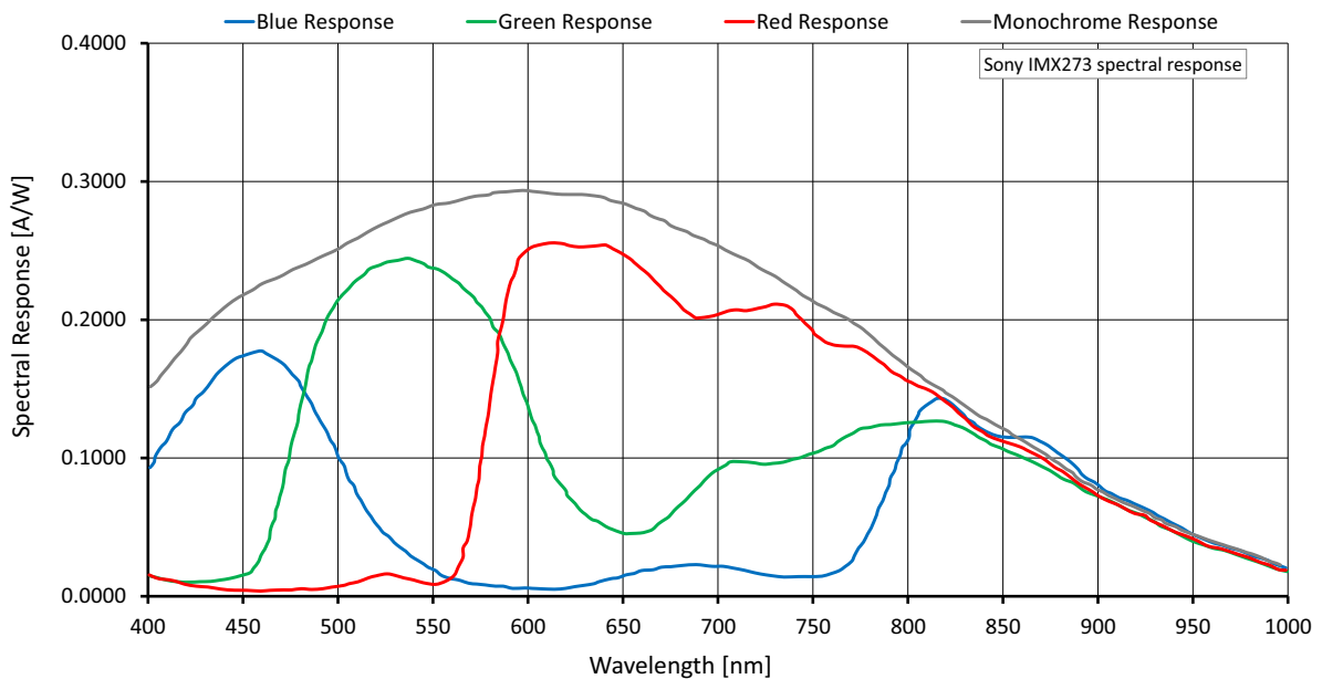
Figure 10: Alvim G1-158m/c (Sony IMX273) spectral response
