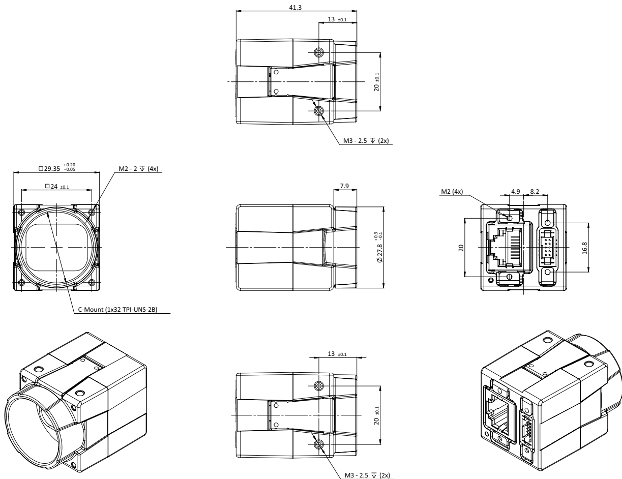
Figure 39: G1 Closed Housing C-Mount dimensions
