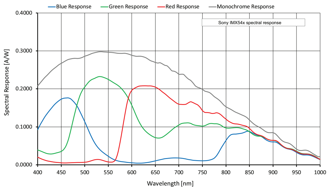
Figure 38: Alvim G1-2460m/c (Sony IMX540) spectral response
