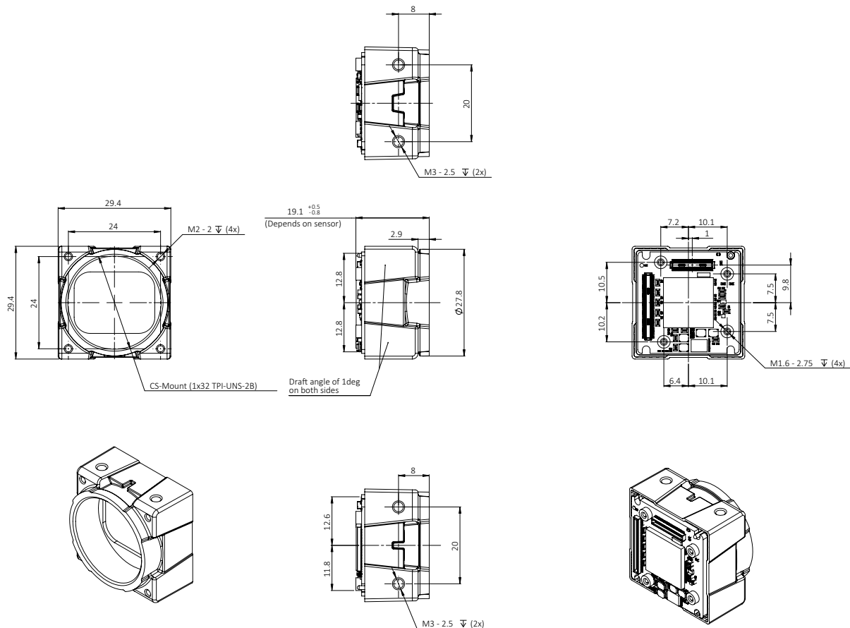
Figure 44: Alvium G1 BL CS-Mount dimensions
