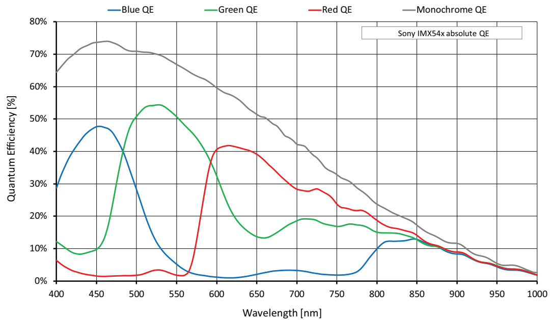
Figure 29: Alvim G1-1242m/c (Sony IMX545) absolute QE
