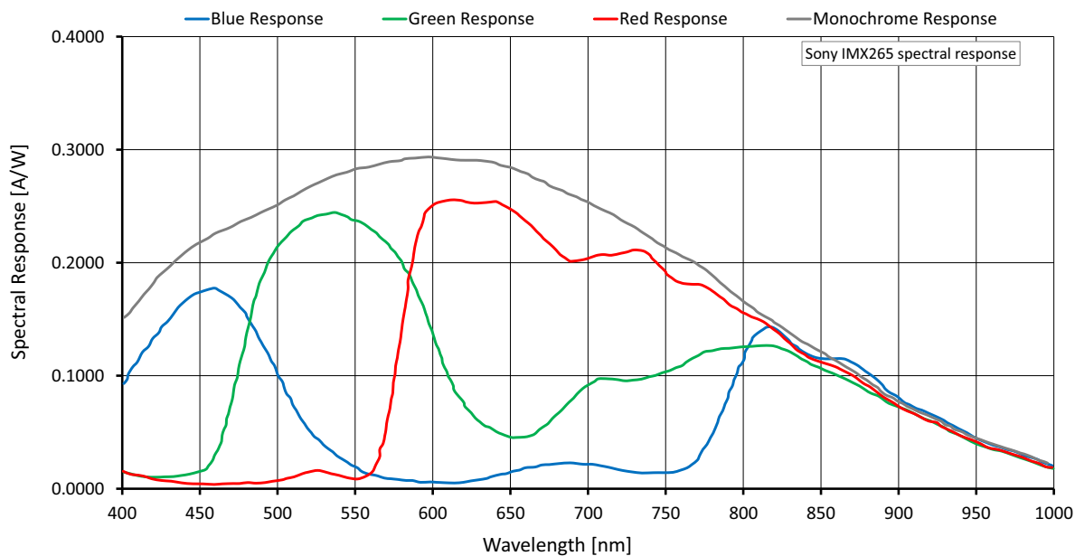
Figure 16: Alvium G1-319m/c (Sony IMX265) spectral response
