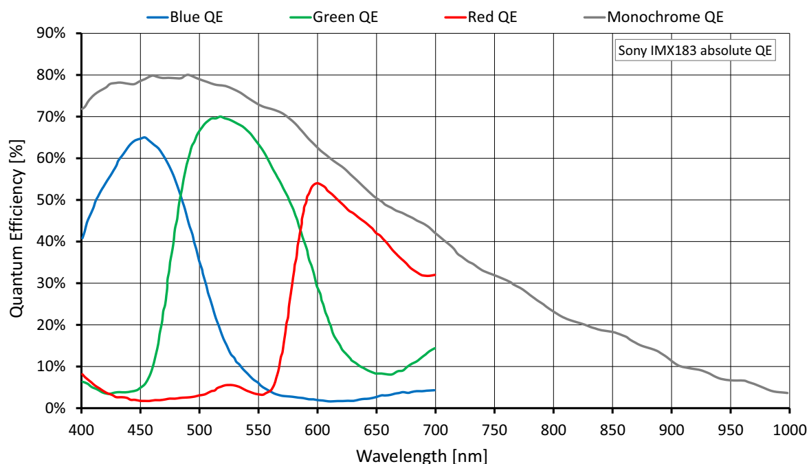
Figure 35: Alvim G1-2050m/c (Sony IMX183) absolute QE
