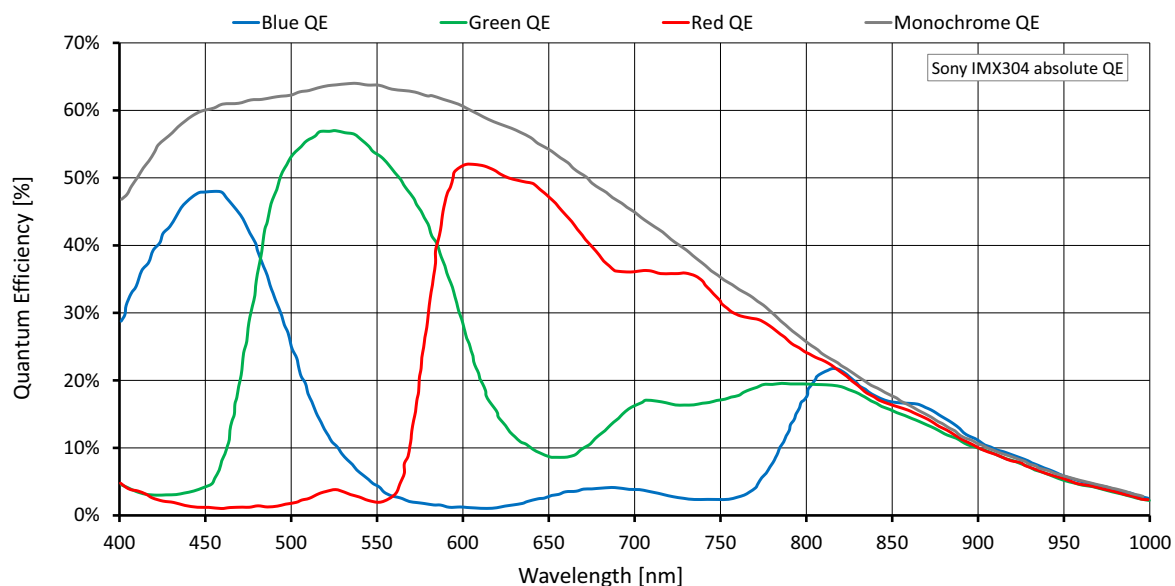
Figure 25: Alvim G1-1236m/c (Sony IMX304) absolute QE
