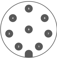
LaserLink Connector: M8 8-Pin A-Coded Female
