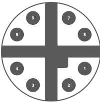
Ethernet Connector: M12 8-Pin X-Coded Female
