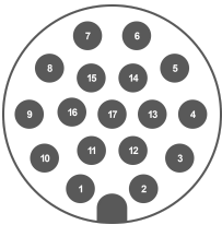
Power & I/O Connector: M12 17-Pin A-Coded Male
