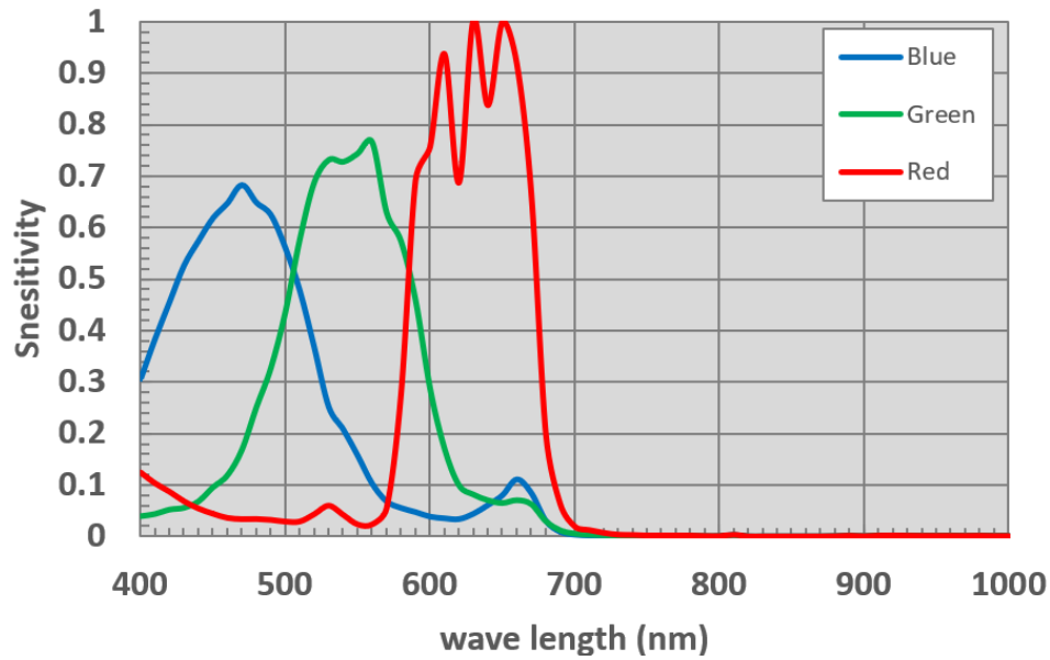
SW-4005 Sensitivity
