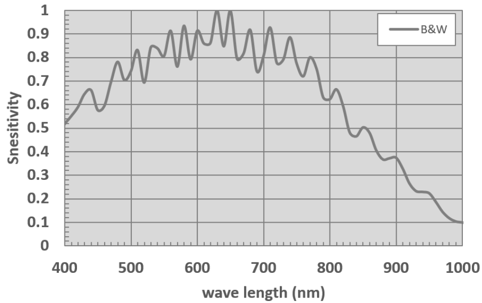
SW-4005 Sensitivity
