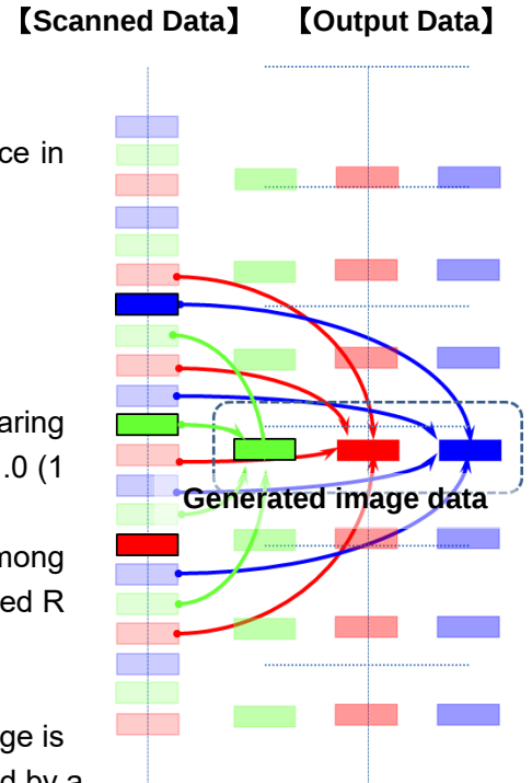
Fig 3.10-7 Line adjustment pixel position (After offsetting Green position)
