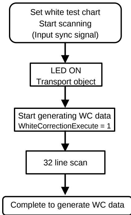
Fig 3.8-1 WC data generation flow (Normal Trigger mode)
