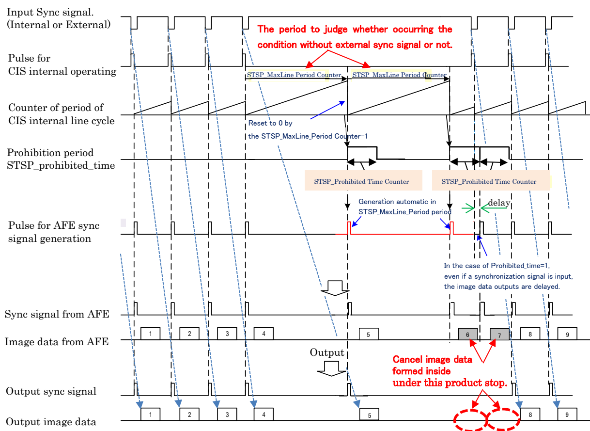
Fig 3.18-1 Timing chart of Prevention for Exposure Saturation
