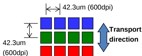
Fig 3.10-1 Color pixel position
