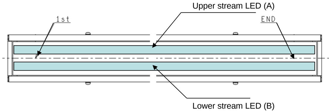
Fig 3.6-1 LED position
