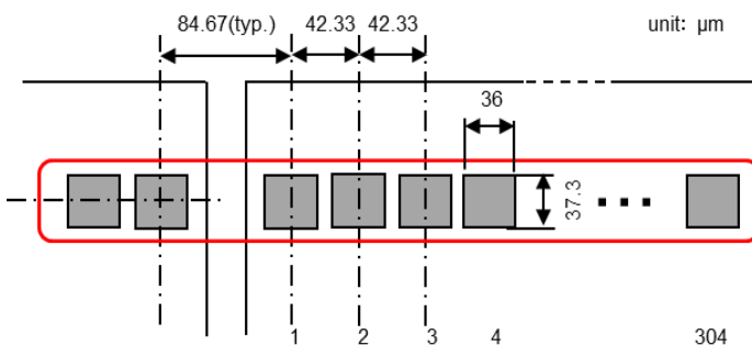
Fig 3.4-2 Pixel alignment of Sensor ICs
