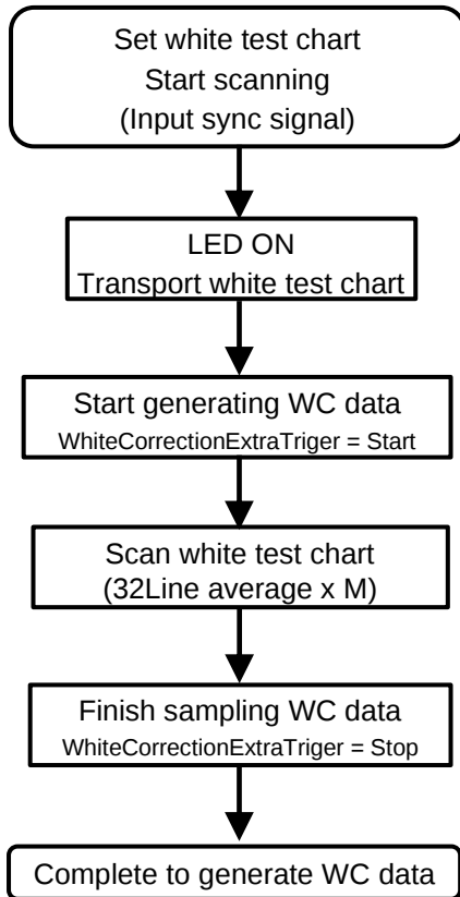
Fig 3.8-3 WC Data generation flow (External Trigger mode)
