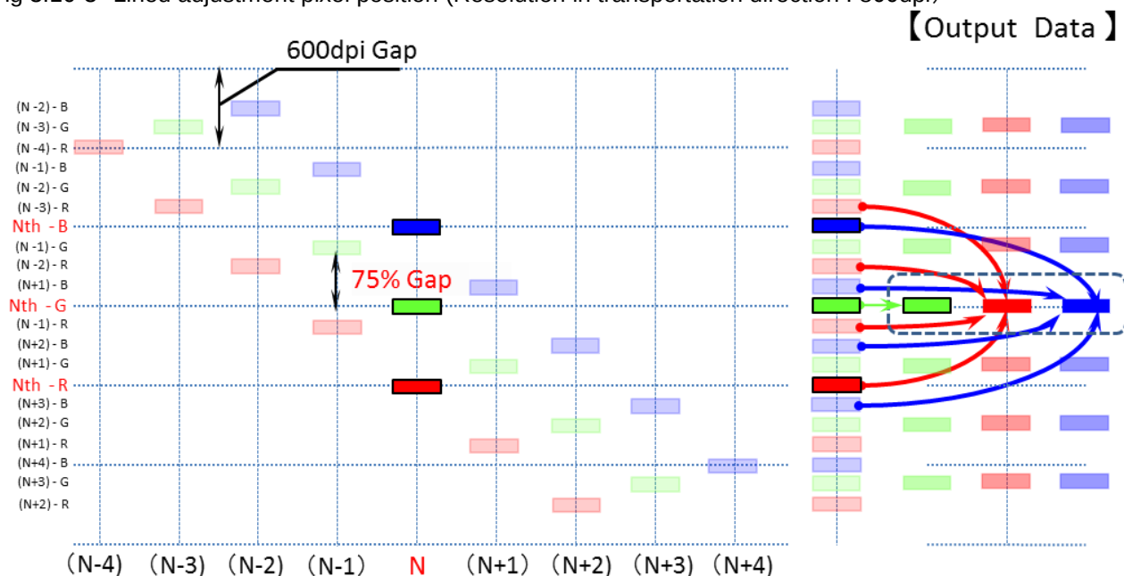
Fig 3.10-3 Lined adjustment pixel position (Resolution in transportation direction : 800dpi)
