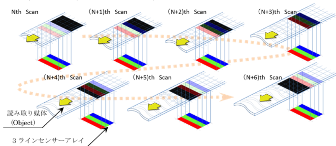
Fig 3.10-2 RGB – Trilinear sensor scanning
