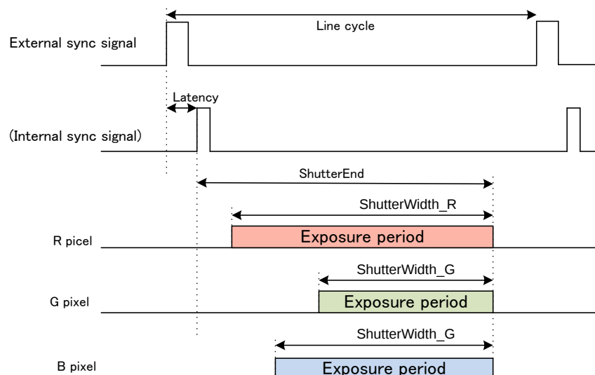
Fig 3.13-1 Electronic shutter timing
