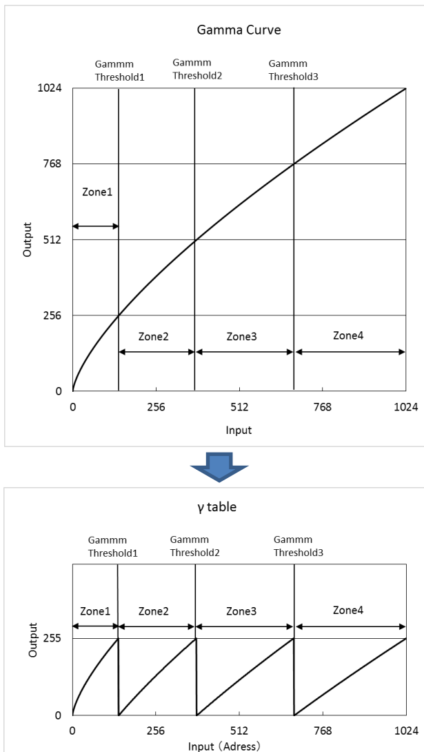
Fig 3.11-1 \gamma curve and \gamma table
