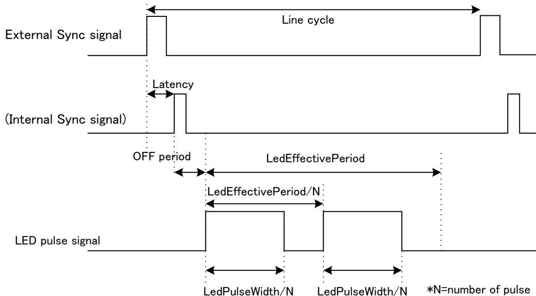
Fig 3.6-3 Division (N=2) LED control pulse timing
