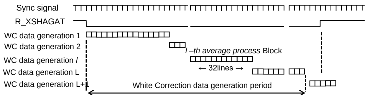
Fig 3.8-4 White Correction data Auto-generation sequence (External Trigger mode(Max hold))理)
