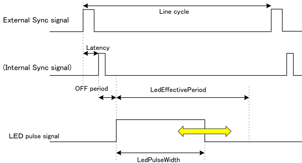
Fig 3.6-2 LED control pulse timing
