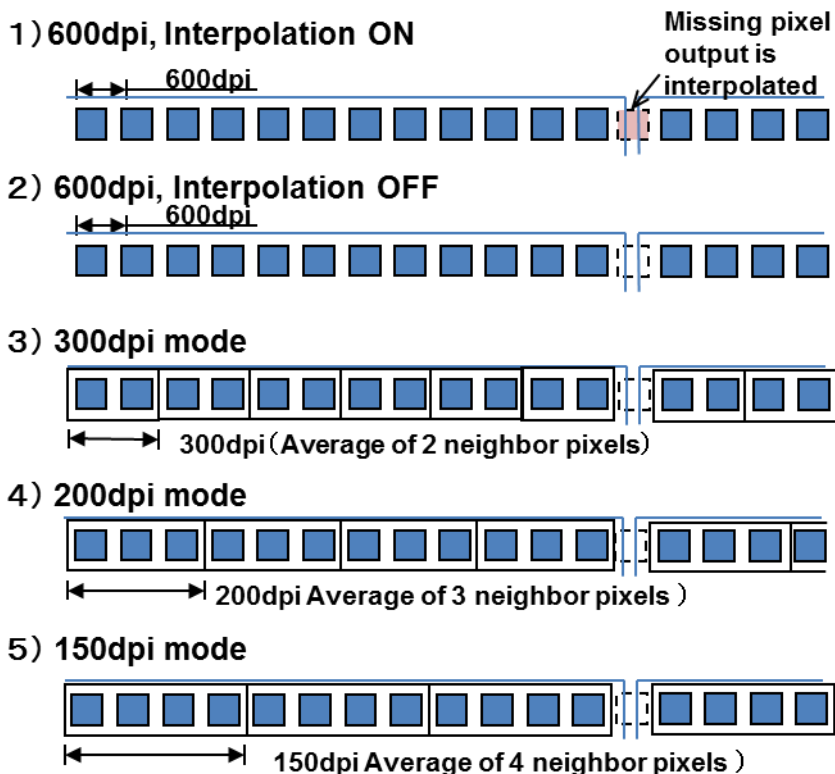
Fig 3.4-1 Output resolution and pixel layout
