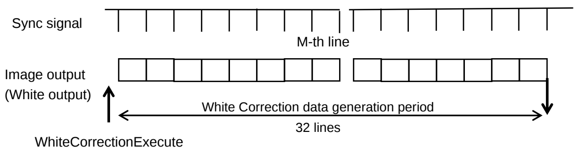
Fig 3.8-2 White Correction Data auto-generation sequence (Normal Trigger mode)
