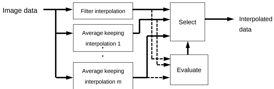
Fig 3.4-4 Interpolation algorithm
