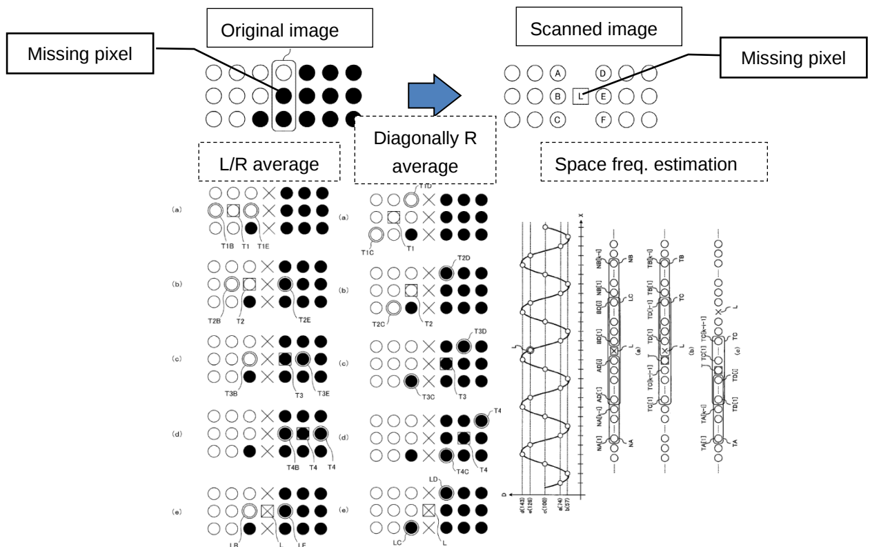
Fig 3.4-4 Interpolation algorithm
