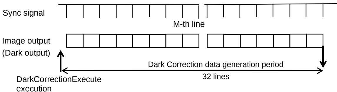
Fig 3.7-2 Dark Correction data auto-generation sequence
