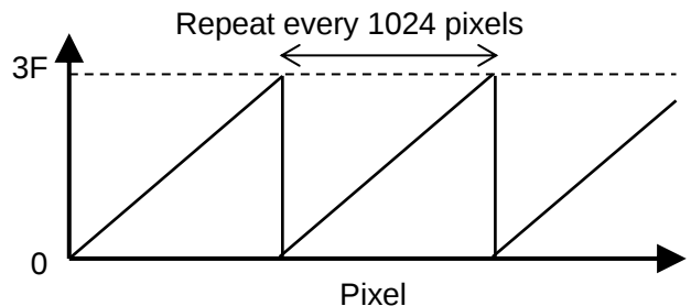
b) Ramp waveform (10bit/pixel output)
