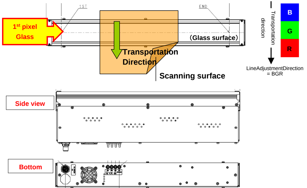
Fig 3.10-6 Product position and transportation direction
