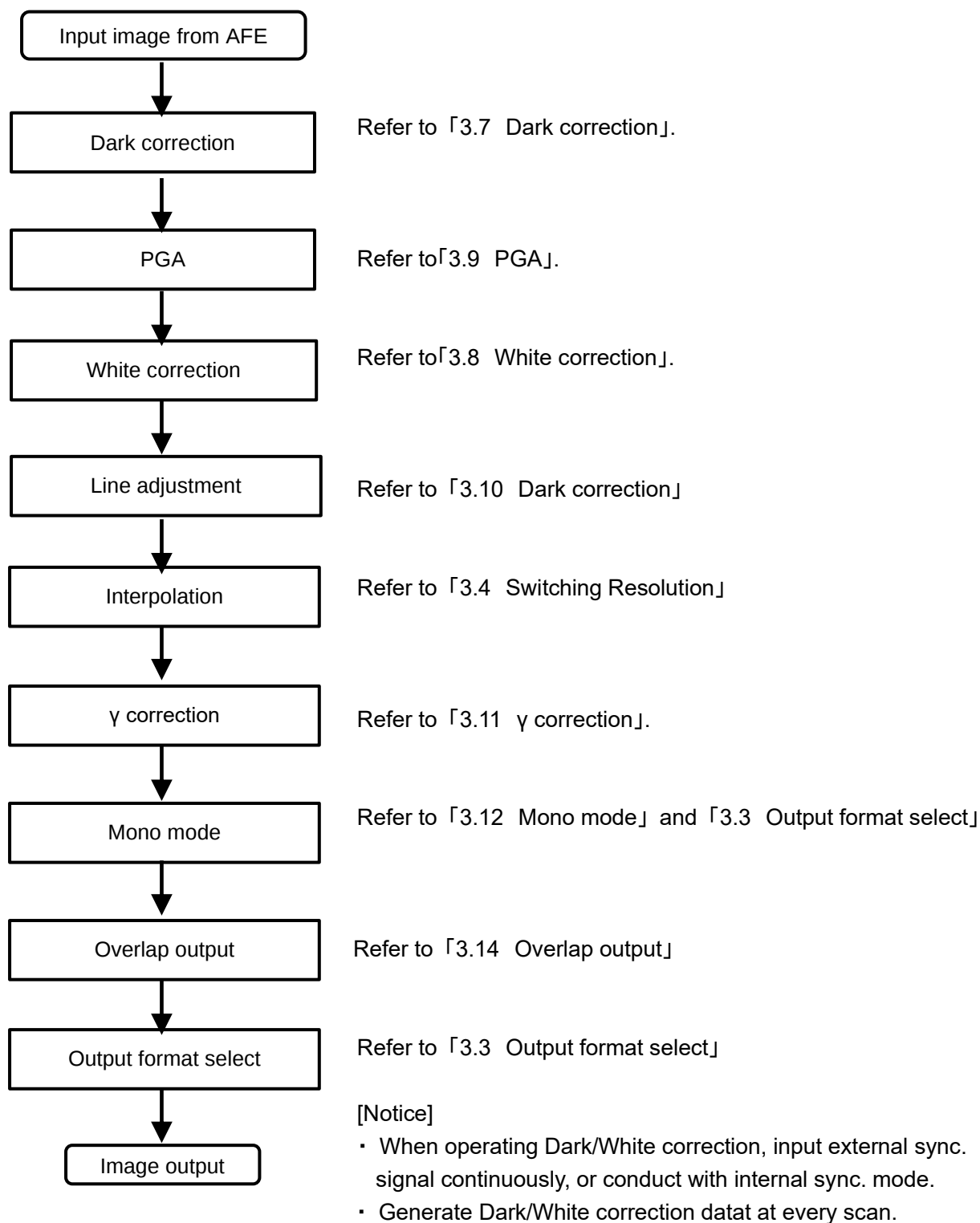
Fig 2.3-1 Image processing flow
