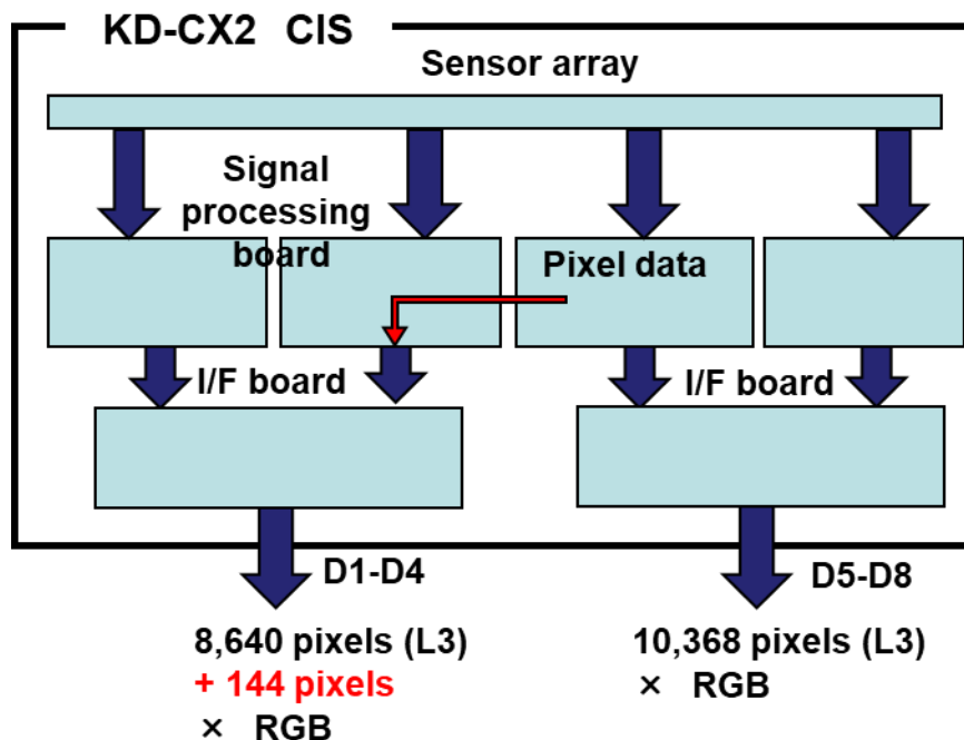
Fig 3.14-1 Function block diagram of Overlap
