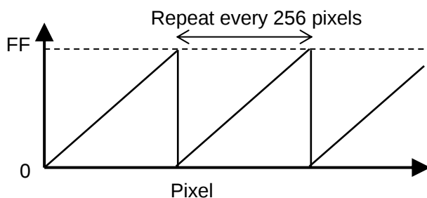
a) Ramp waveform (8bit/pixel output)
