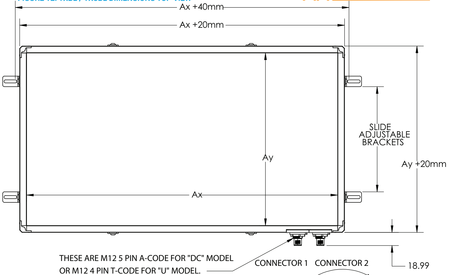
FIGURE 13: TXBL / TXCBL DIMENSIONS SIDE VIEW
