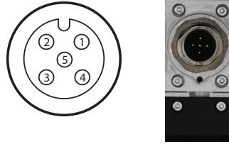
FIGURE 1: TXBL INTERFACE CABLE, M12 5-PIN A-CODE FEMALE CONNECTOR
