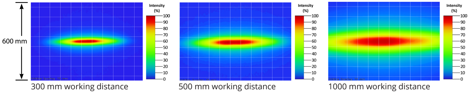
Line (10° x 50°) beam patterns Grid set to 75 mm
