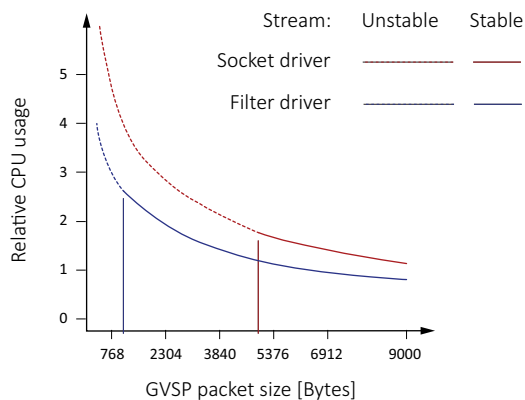
Figure 98: GVSPPacketSize versus CPU usage while the camera is streaming
