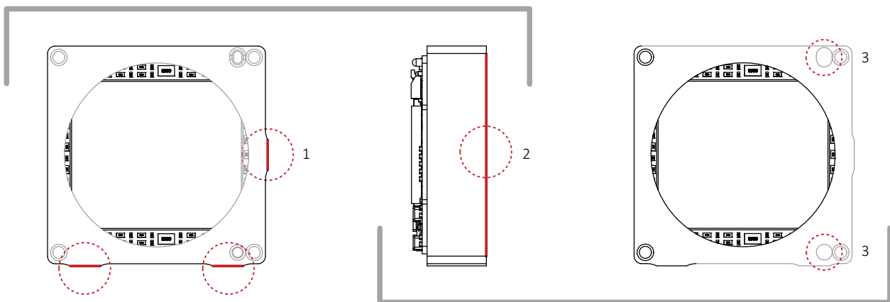
Figure 64: Alignment methods
