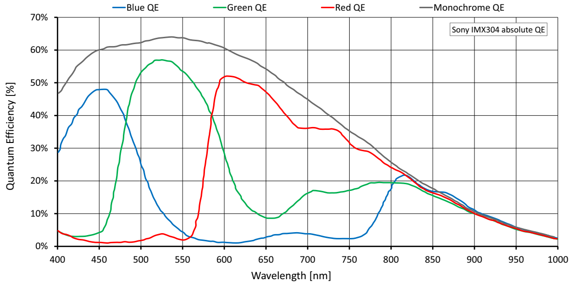
Figure 30: Alvium G1-1236m/c (Sony IMX304) absolute QE
