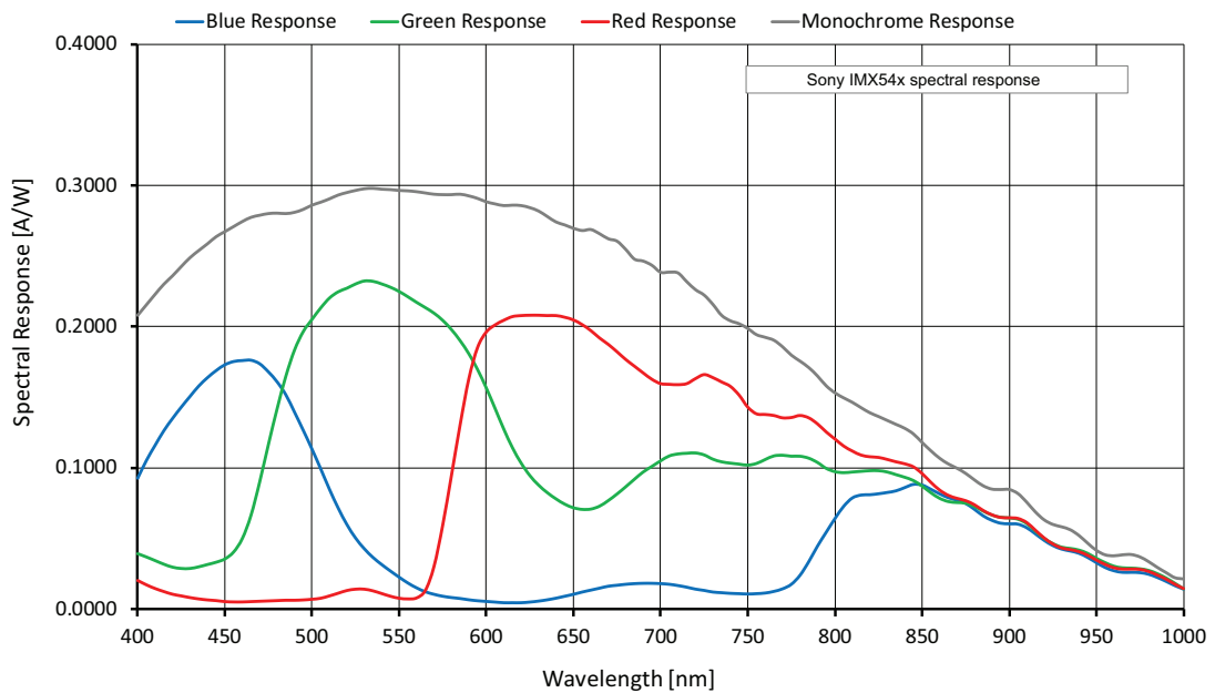
Figure 37: Alvium G1-1620m/c (Sony IMX542) spectral response
