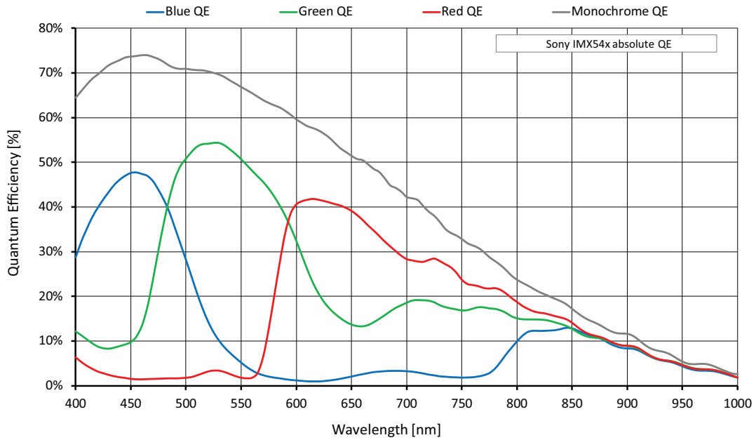
Figure 38: Alvium G1-2040m/c (Sony IMX541) absolute QE
