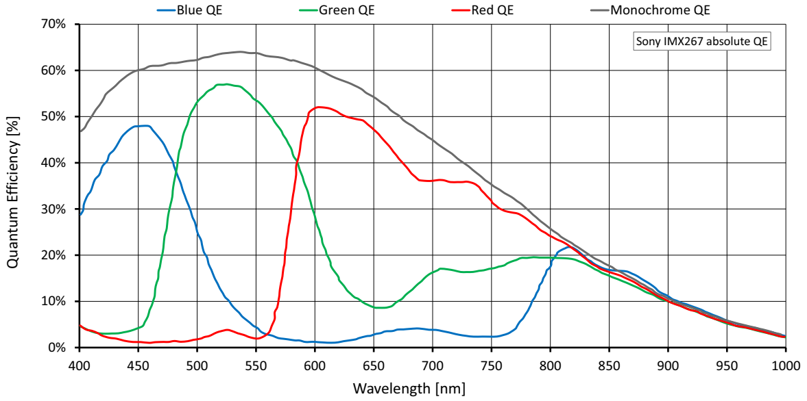
Figure 28: Alvium G1-895m/c (Sony IMX267) absolute QE
