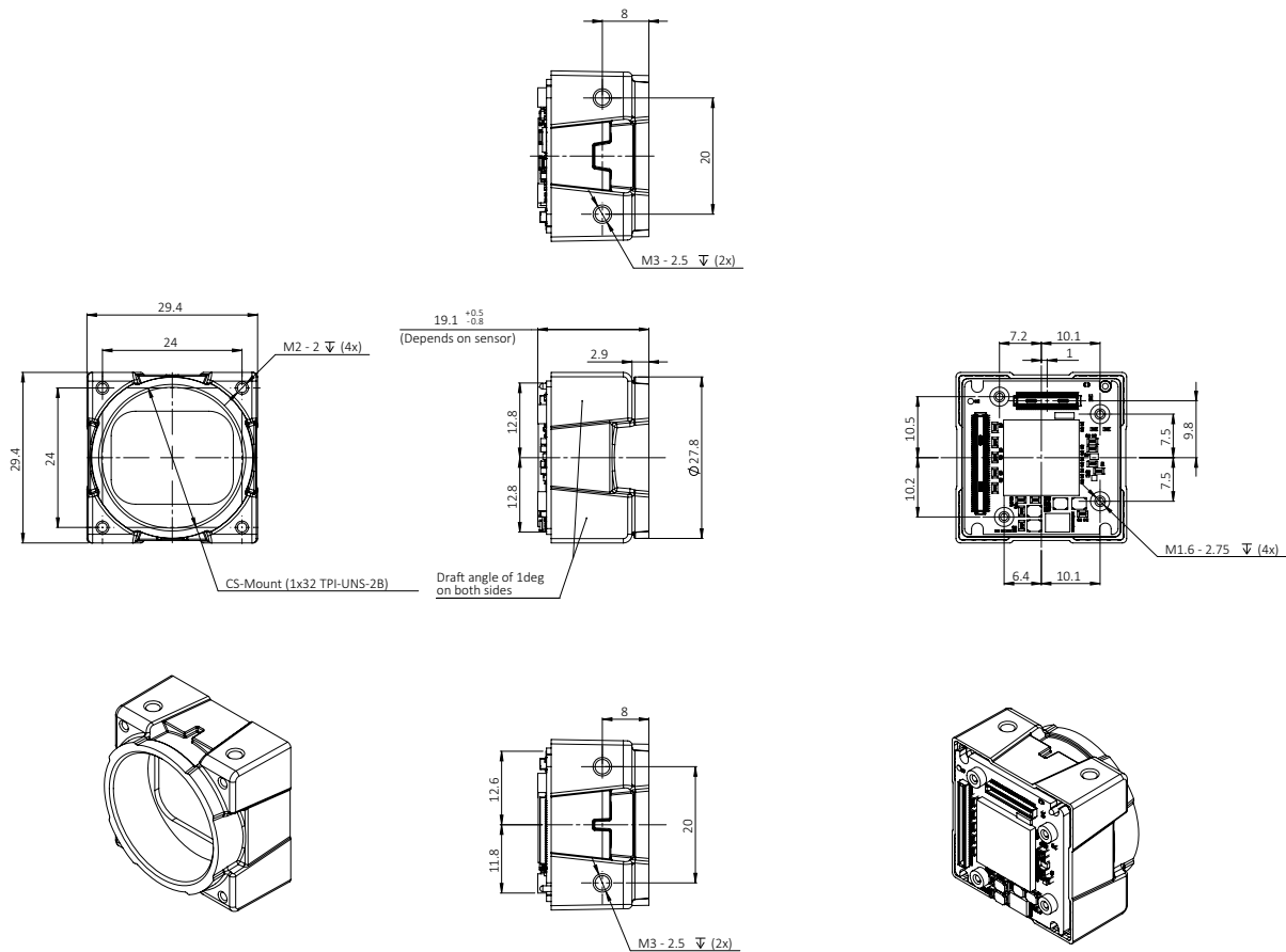
Figure 48: Alvium G1 BL CS-Mount dimensions
