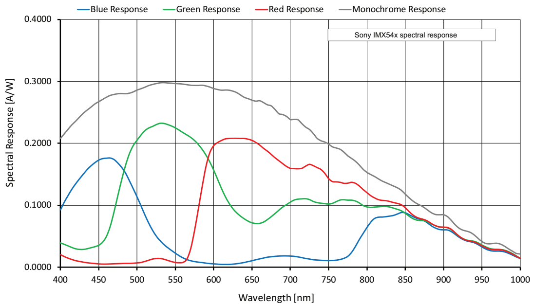
Figure 39: Alvium G1-2040m/c (Sony IMX541) spectral response
