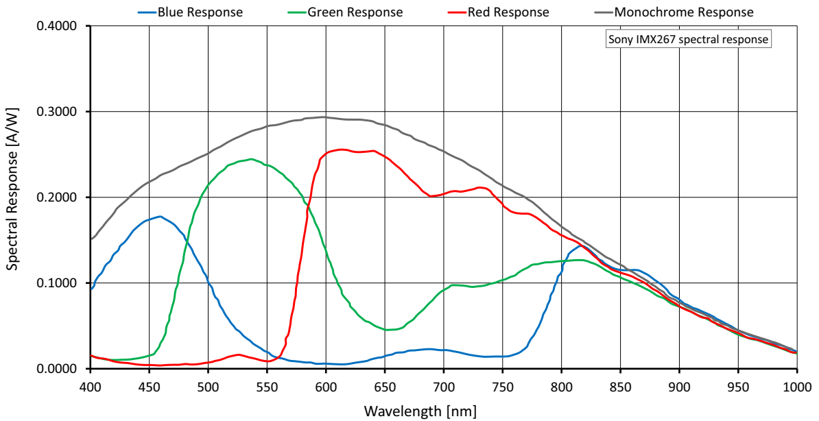
Figure 29: Alvium G1-895m/c (Sony IMX267) spectral response
