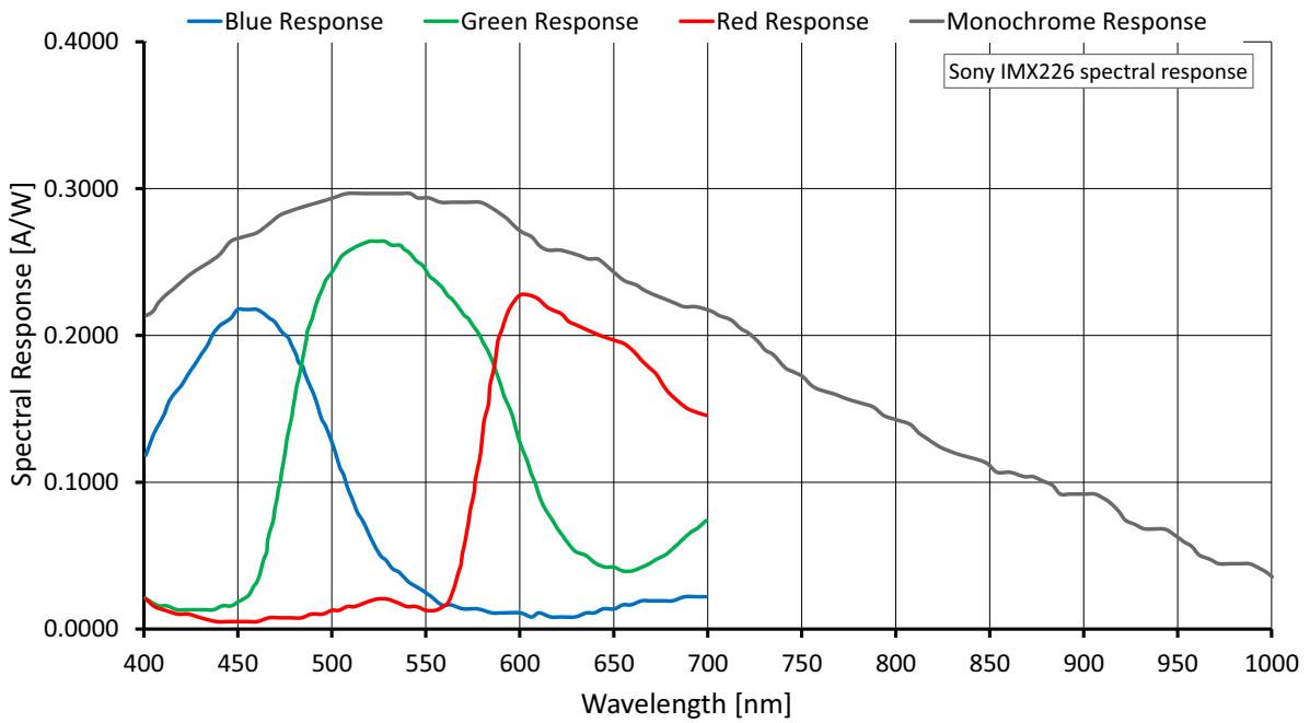
Figure 33: Alvium G1-1240m/c (Sony IMX226) spectral response
