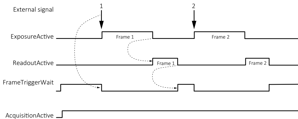
Figure 86: Schematic trigger signal flow
