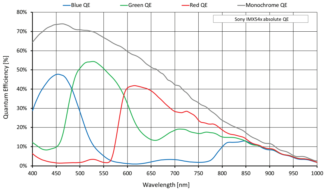
Figure 42: Alvium G1-2460m/c (Sony IMX540) absolute QE
