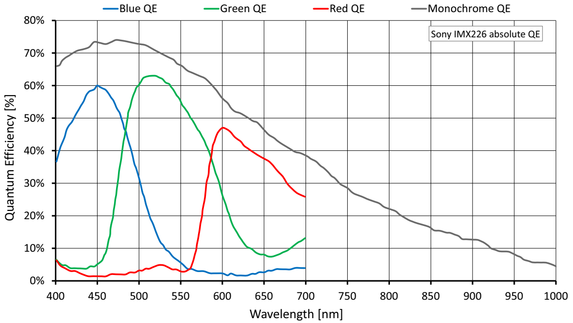
Figure 32: Alvium G1-1240m/c (Sony IMX116) absolute QE
