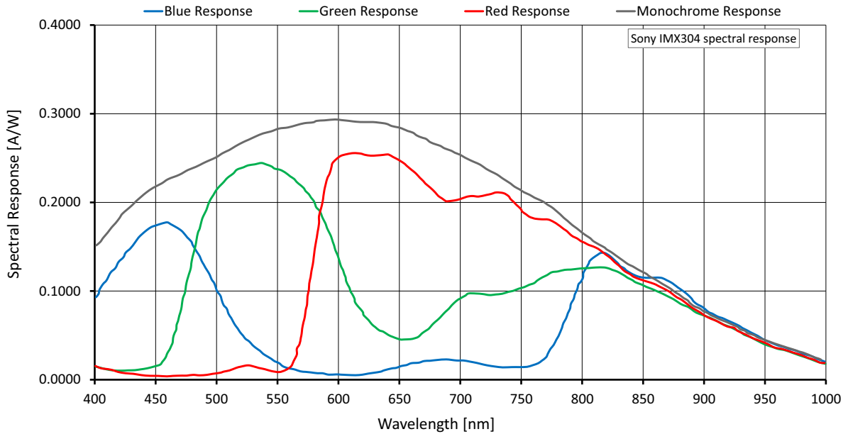
Figure 31: Alvium G1-1236m/c (Sony IMX304) spectral response
