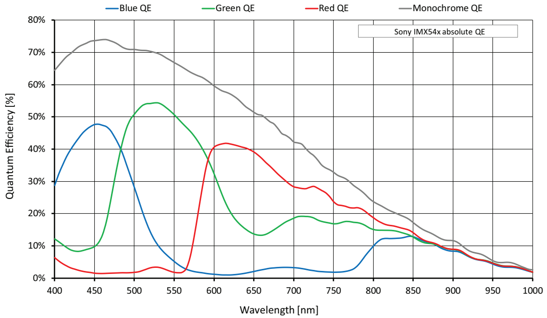
Figure 36: Alvium G1-1620m/c (Sony IMX542) absolute QE
