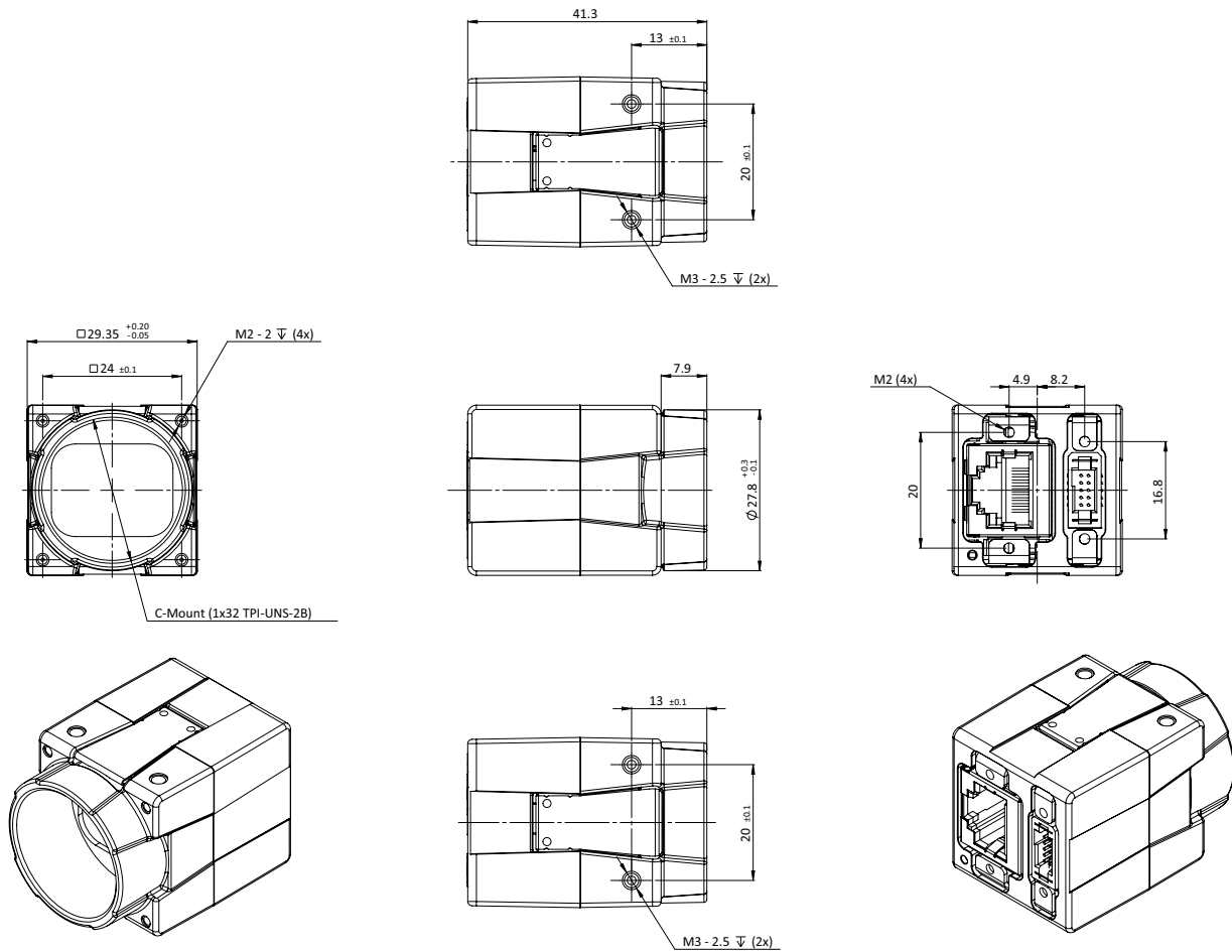
Figure 44: G1 Closed Housing C-Mount dimensions
