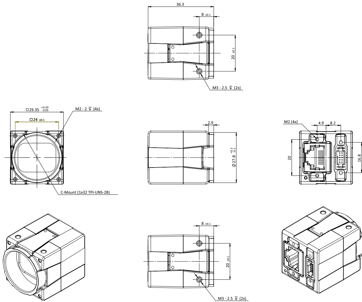
Figure 45: G1 Closed Housing CS-Mount dimensions
