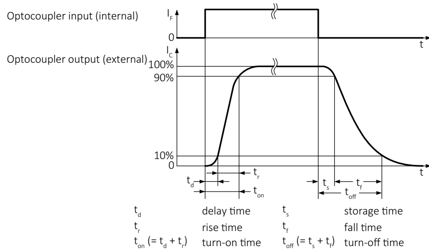
Figure 60: Output switching times
