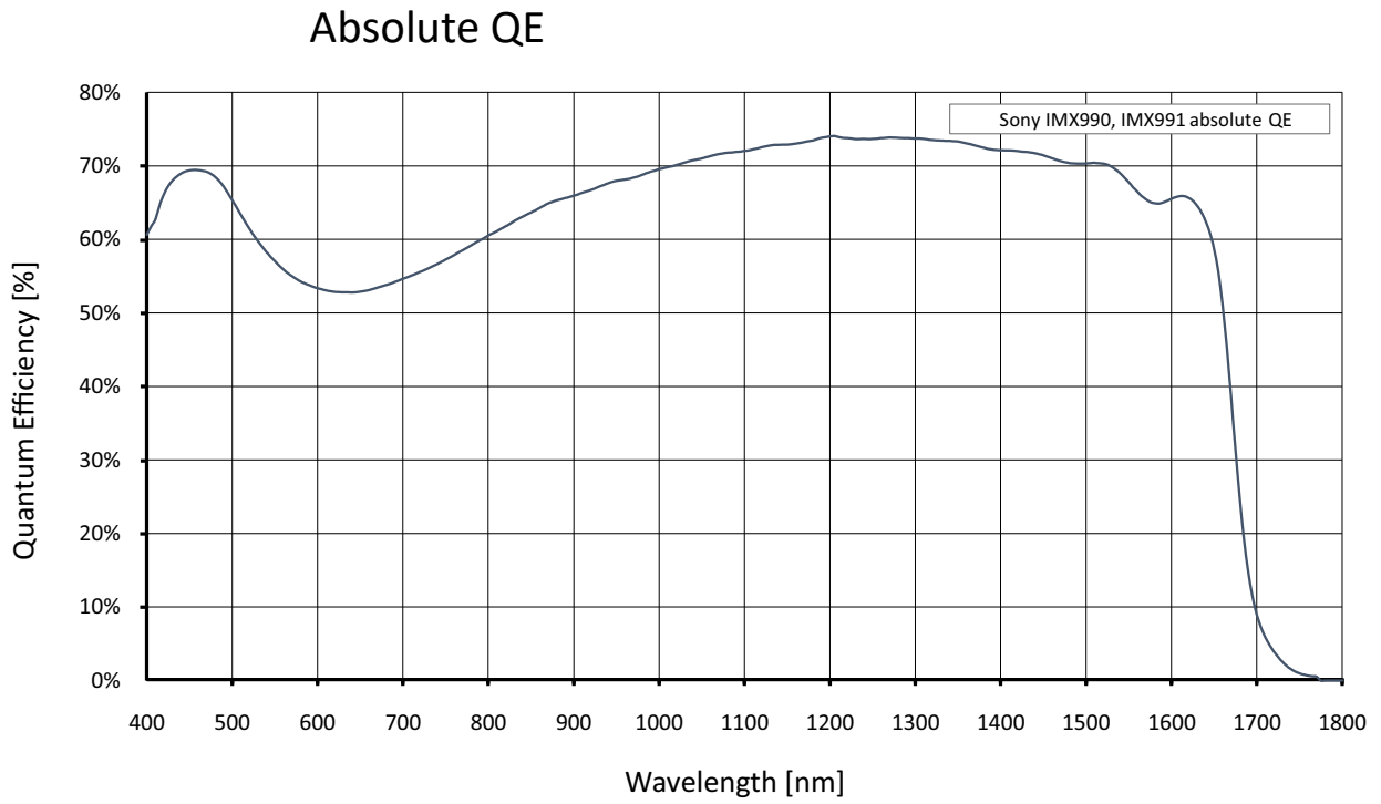
Figure 6: Alvium G5-130m SWIR (Sony IMX990) absolute QE
