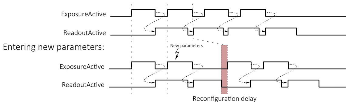
Figure 76: Delayed exposure due to parameter changes
