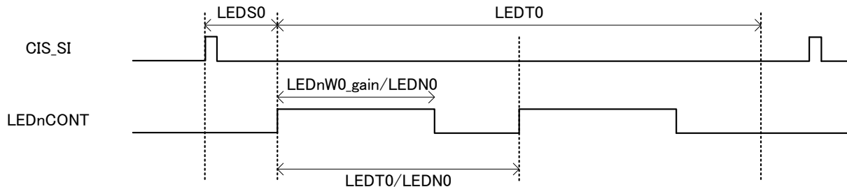
Timing diagram of LED lighting control
